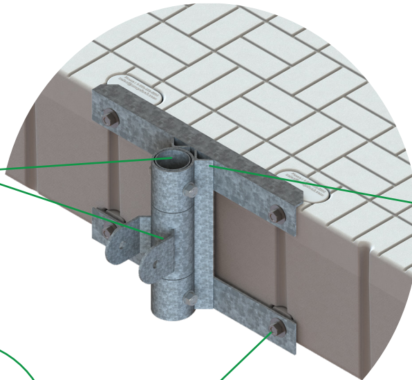
Stiff Arm Adapter
